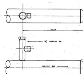
No.12 TYPICAL INSTALLATION OF A PURGING POINT
