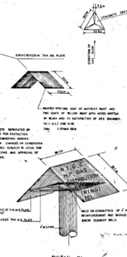
No.12 TYPICAL INSTALLATION OF A PURGING POINT
