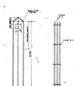
No.11 TYPICAL MARKERS
