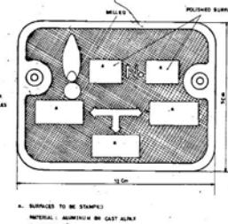
No.10 VALVE INDICATOR PLATE
