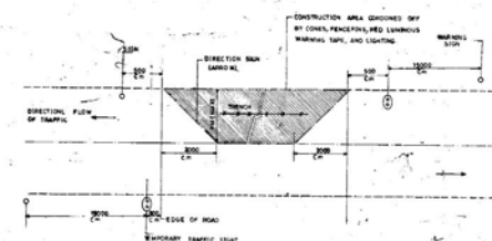
No.13 SPACING AND ARRANGEMENT OF ROAD SIGNS FOR GAS PIPELINE CONSTRUCTION (SINGLE CARRIAGEWAY ROAD)
