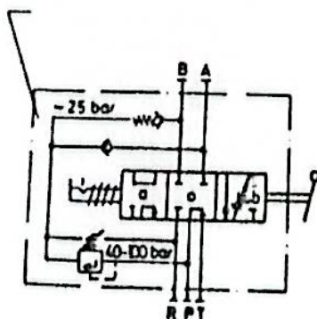
Circuit-diagram for type SS 5/3 A100A
