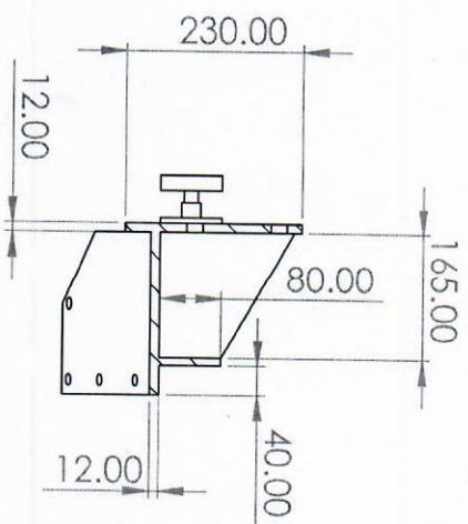
SECTION H-I
